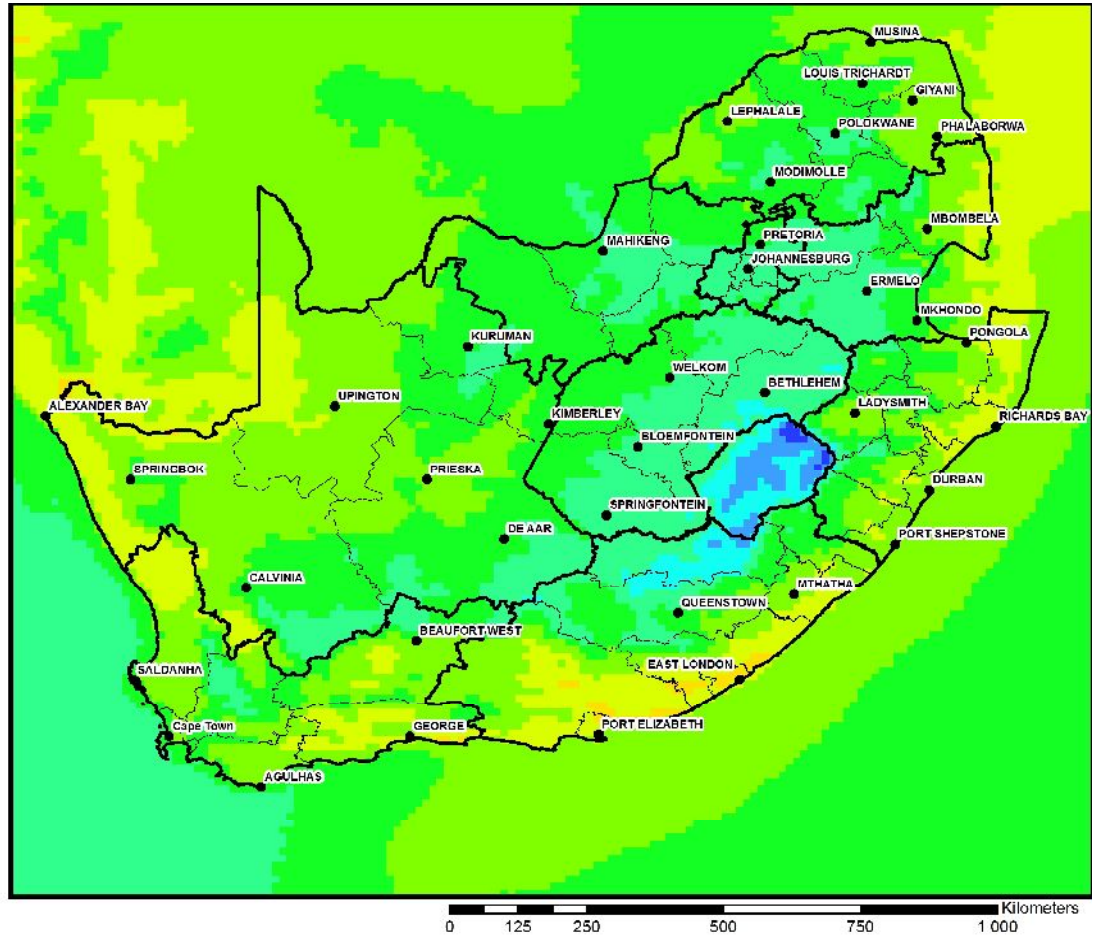
Figure 3: Average Maximum Temperatures: 17 to 23 July 2018.
