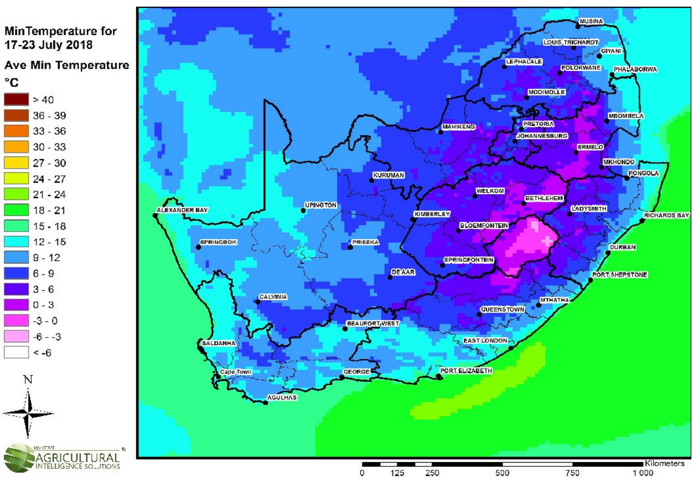
Figure 2: Average Minimum Temperatures: 17 to 23 July 2018.
