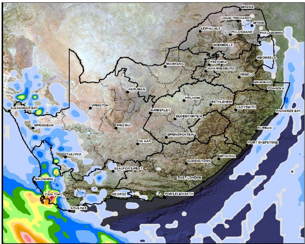
Figure 1: Expected precipitation: 17 to 23 July 2018.
