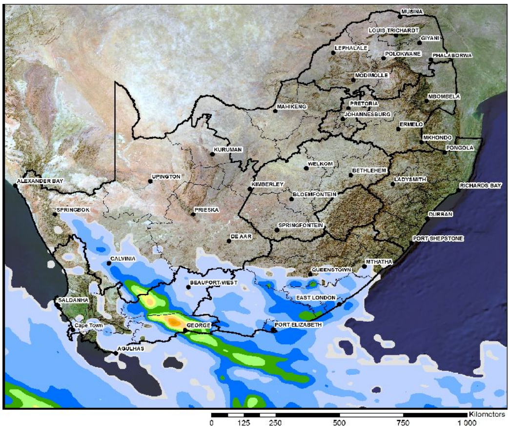
Figure 1: Expected precipitation: 24 to 30 July 2018.
