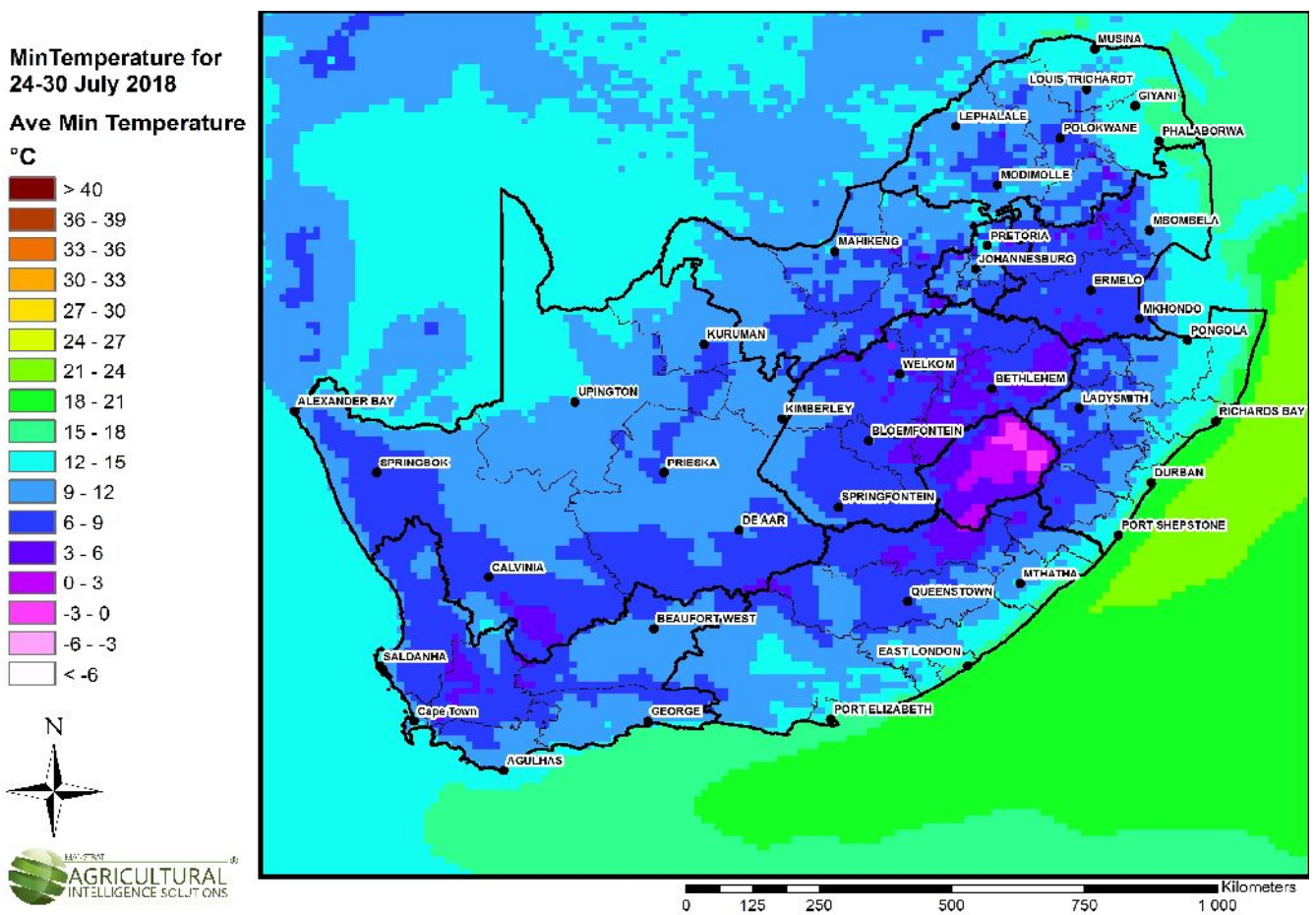
Figure 2: Average Minimum Temperatures: 24 to 30 July 2018.
