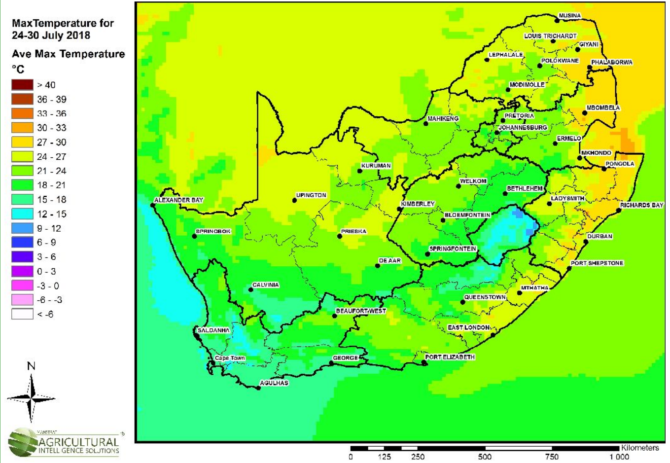
Figure 3: Average Maximum Temperatures: 24 to 30 July 2018.
