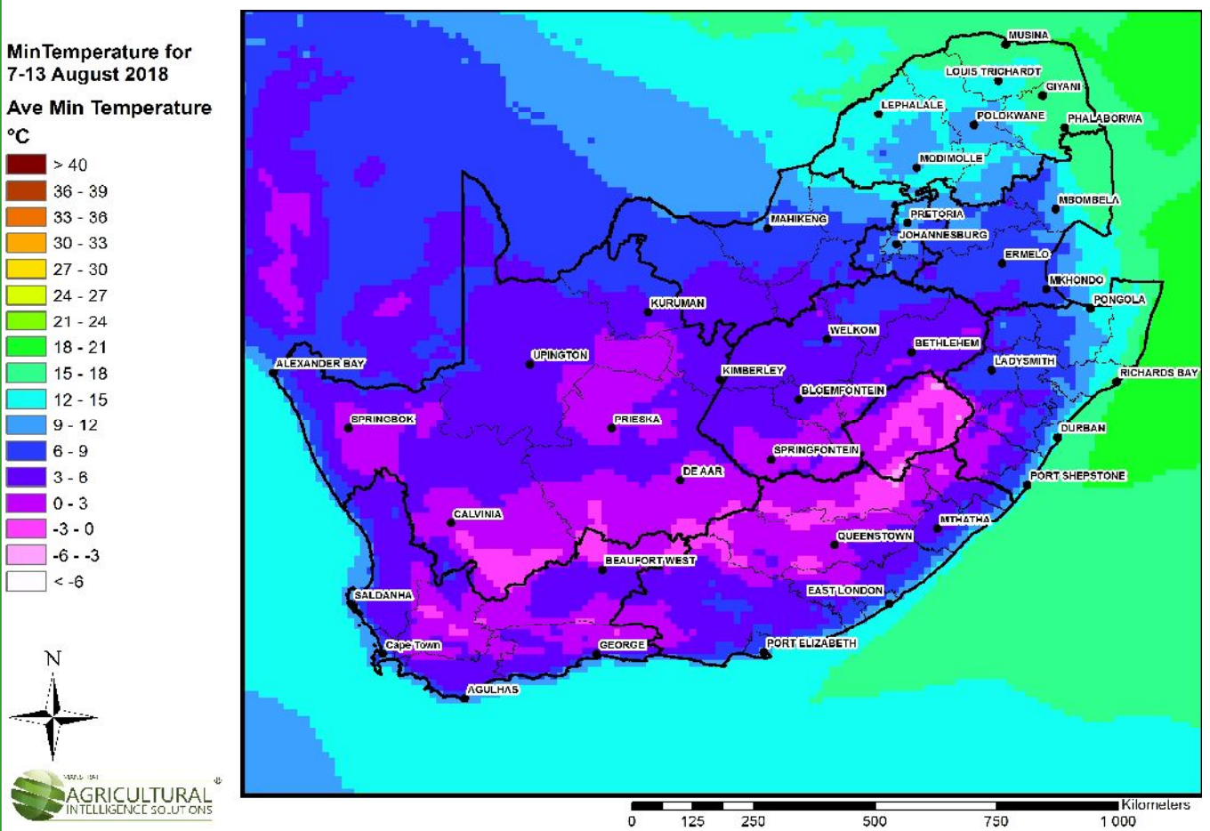
Figure 2: Average Minimum Temperatures: 7 to 13 August 2018.
