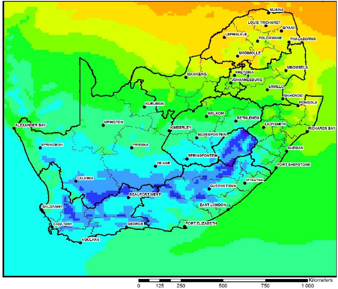
Figure 3: Average Maximum Temperatures: 7-13 August 2018.
