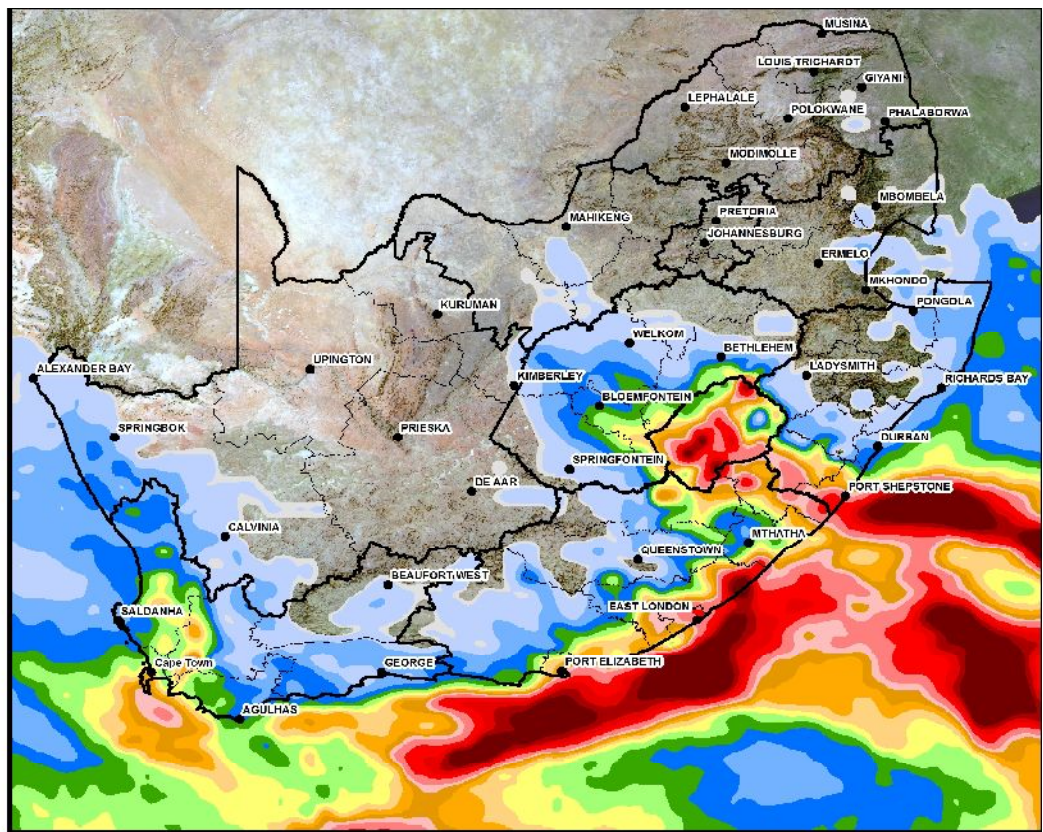
Figure 1: Expected precipitation: 7 to 13 August 2018.
