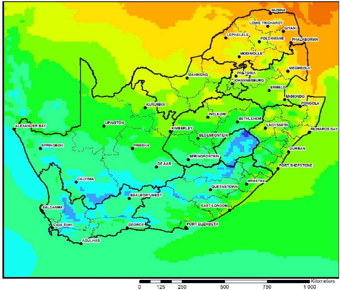
Figure 3: Average Maximum Temperatures: 21 to 27 August 2018.
