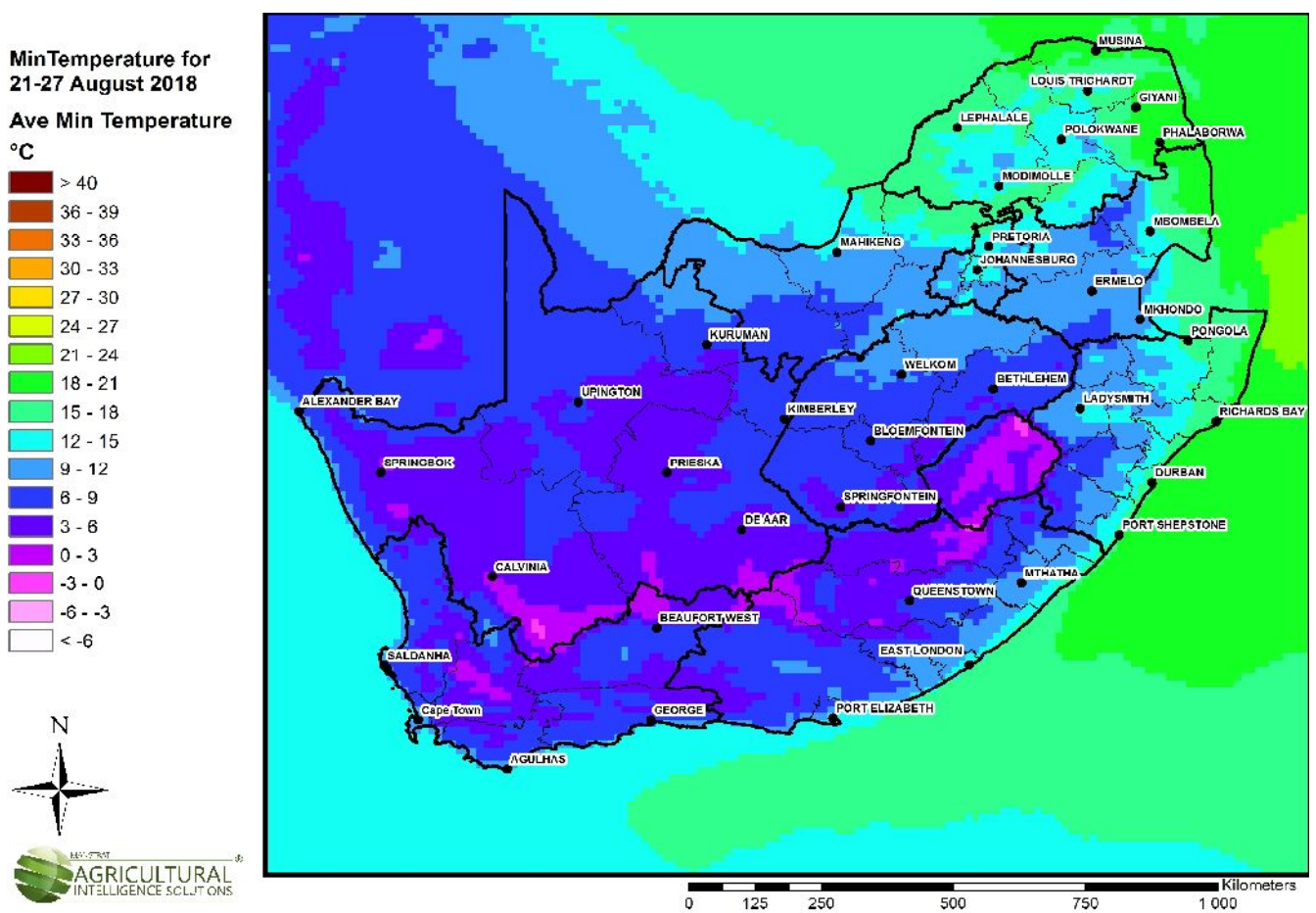
Figure 2: Average Minimum Temperatures: 21 to 27 August 2018.
