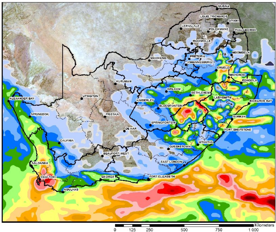
Figure 1: Expected precipitation: 21 to 27 August 2018.
